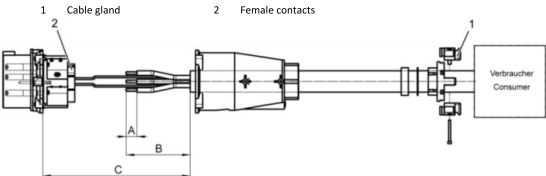
Fig.7: Schematic for cables with integrated pilot contacts
