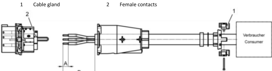
Fig.6: Schematic for cables without pilot contacts
