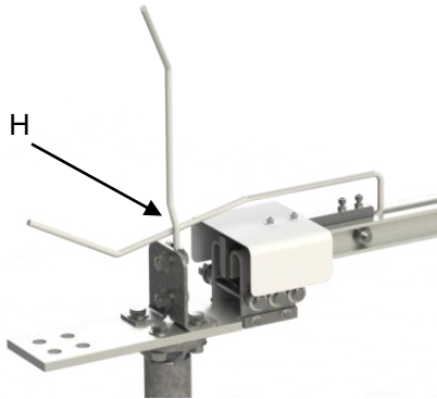
Fig. 29: Arcing horns
