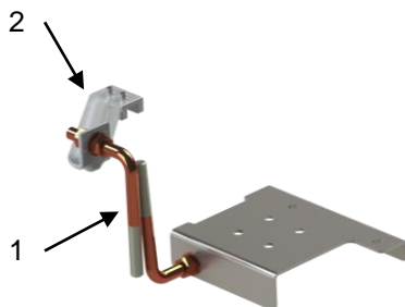
Fig. 20: Pre-arcing horns
