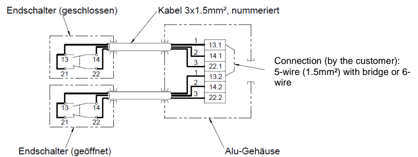
Fig. 24: Wiring diagram
