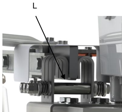
Fig. 27: Main contact
