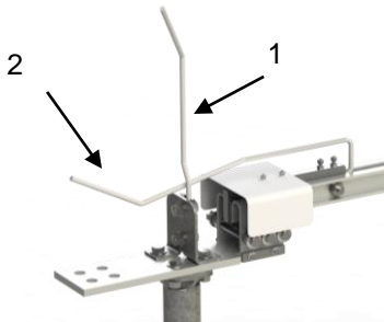
Fig. 14: Arcing horns
