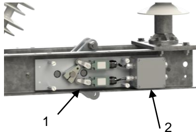
Fig. 18: Status indication
