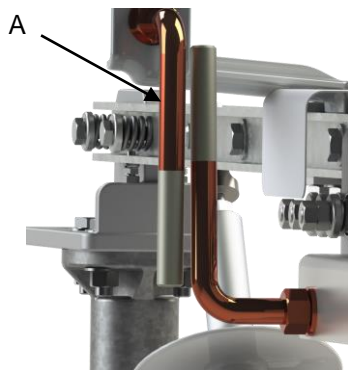
Fig. 30: Pre arcing horns
