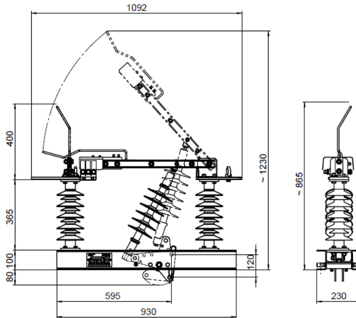
Fig. 4: FHF-B3-15/S dimensions
