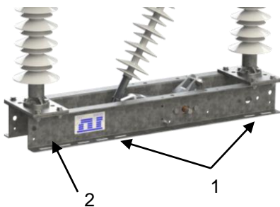
Fig. 22: Fastening & earthing
