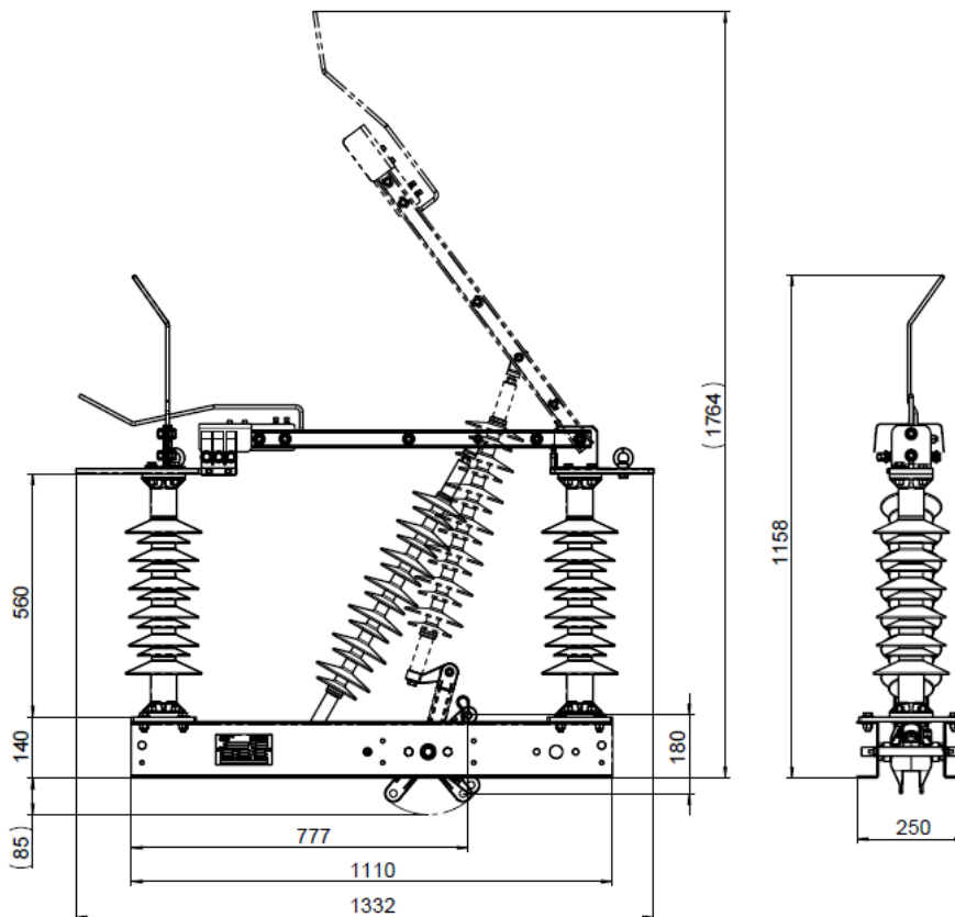
Fig. 5: FHF-B3-25/S dimensions
