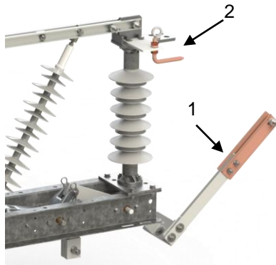
Fig. 19: Forced earthing
