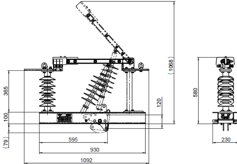
Fig. 6: FHE-B3-15/S dimensions
