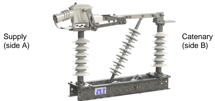
Fig. 26: Installation direction (example FHV-B3)
