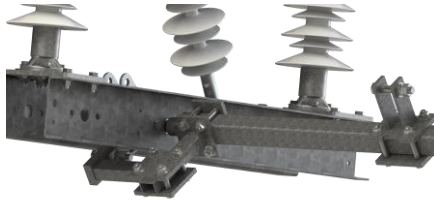
Fig. 23: Installation of the coupling kit
