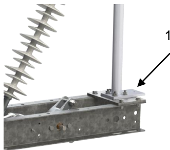
Fig. 25: Earth connection
