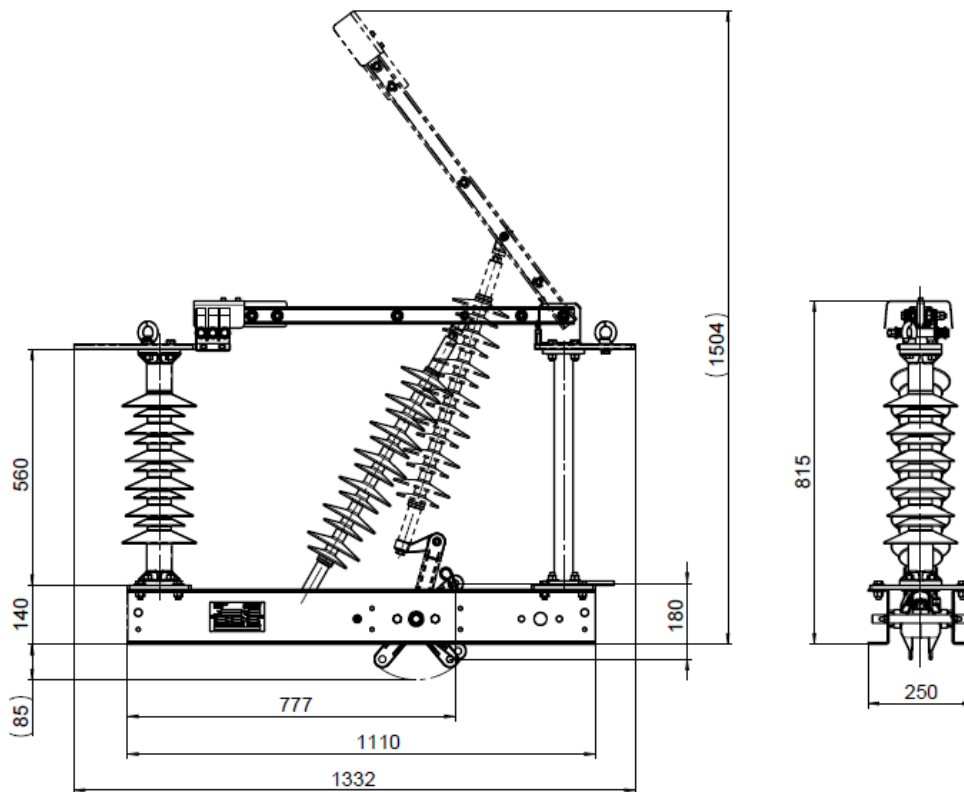
Fig. 7: FHE-B3-25/S dimensions
