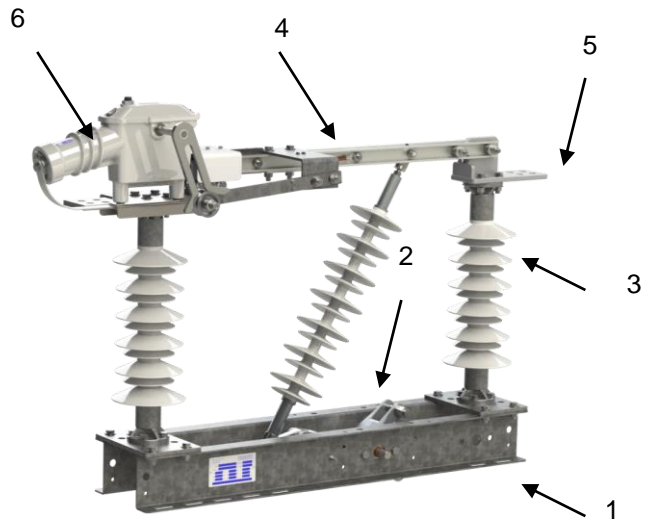
Fig. 8: Basic design (example: FHV-B3)
